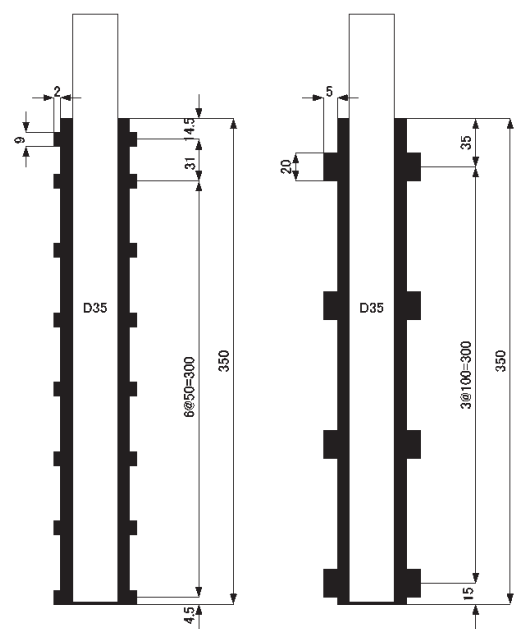
(a) 溝タイプA
